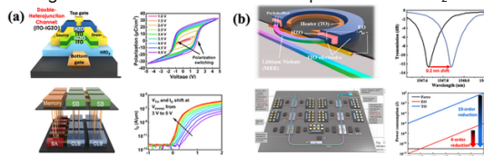
Fig. 2: (a) HZO-IGZO Dual-Gate Memtransistor and the transistor's non-volatile ferroelectric memory switching characteristics, with proposed application for BEOL-integrated switch matrix for non-volatile FPGA [4]. (b) HZO-Lithium Niobate Micro Ring Resonator (MRR), Electro-Optic Modulator and Memory with non-volatile photonic memory operations and energy reduction gains with respect to thermal-modulated MRR. We proposed it as a non-volatile switch for reconfigurable photonic inter-chip let interconnect system [5].
